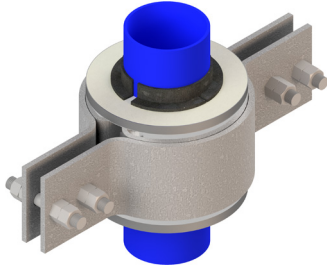
Polyurethane Riser (Low Load)
