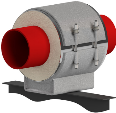
Calcium Silicate Resting
