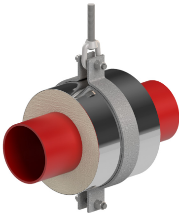
Calcium Silicate Hanging (Low Load)
