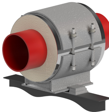
Calcium Silicate Vertically Restrained Guided
