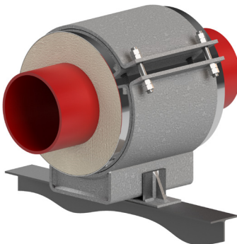
Calcium Silicate Guided
