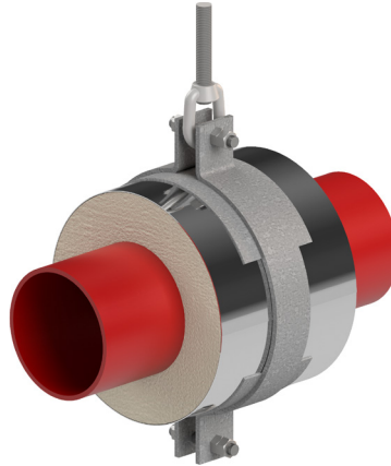
Calcium Silicate Hanging (Medium Load)
