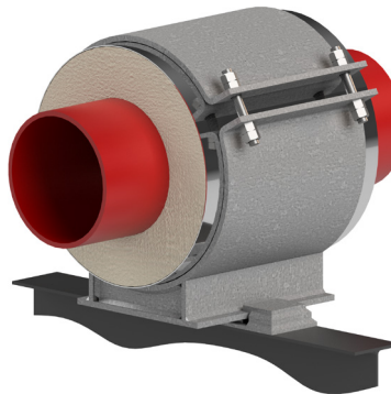
Calcium Silicate Vertically Restrained Guided
