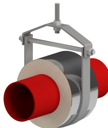
Calcium Silicate Roller (High Load)
