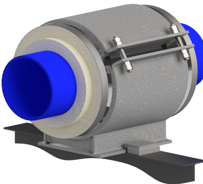
Polyurethane Vertically Restrained Guided
