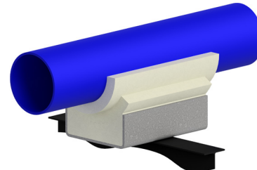
Polyurethane Insulated Guided (180 degree) Double Layer
