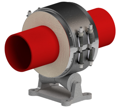
Calcium Silicate Roller (High Load)
