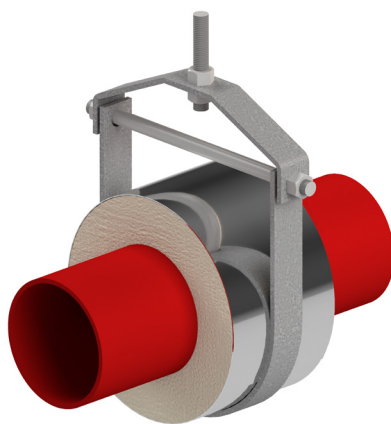
Calcium Silicate Roller (Low Load)
