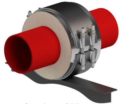
Calcium Silicate Flat (High Load)
