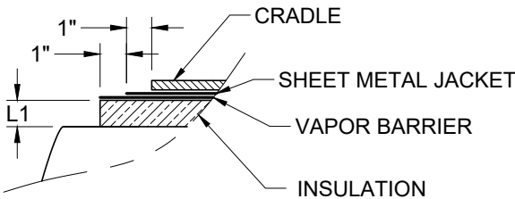
SINGLE LAYER
