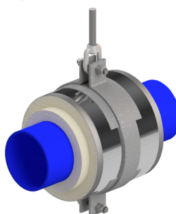
Polyurethane Hanging (Medium Load)
