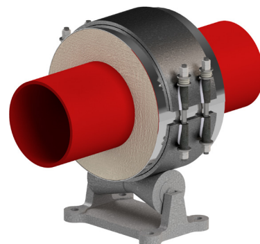
Calcium Silicate Roller (High Load)
