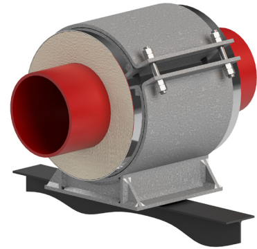
Calcium Silicate High Lateral Travel
