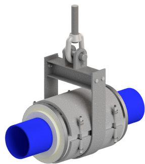
Polyurethane Hanging (High Load)
