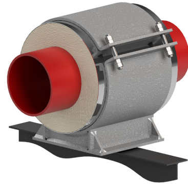
Calcium Silicate High Lateral Travel
