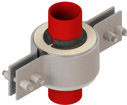
Calcium Silicate Riser (Low Load)
