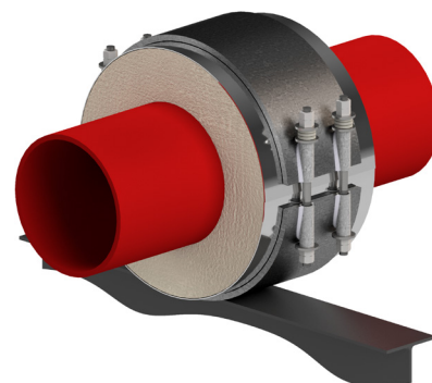
Calcium Silicate Flat (High Load)
