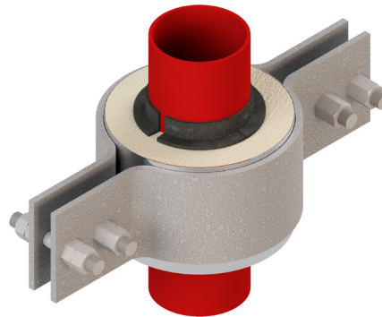
Calcium Silicate Riser (High Load)
