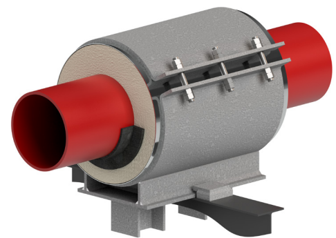
Calcium Silicate Anchor
