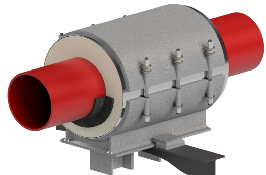
Calcium Silicate Anchor
