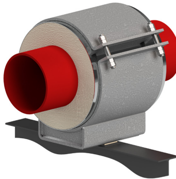
Calcium Silicate Resting- Bent Ear
